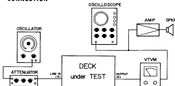
Fig. 7-22 Connection
