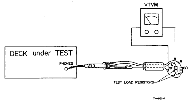
Fig. 7-6 Connection
