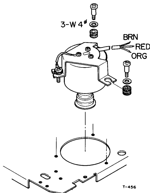
Fig. 3-2 Motor Replacement
