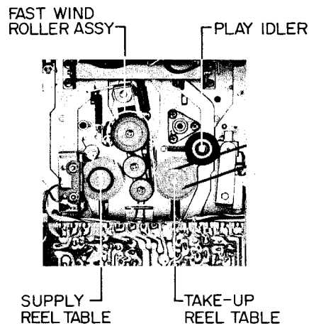
Fig. 5-1 Bottom View w/Flywheel Removed
