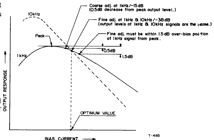
Fig. 7-12 Bias Adjustments (CrO 2 & FeCr tapes)
