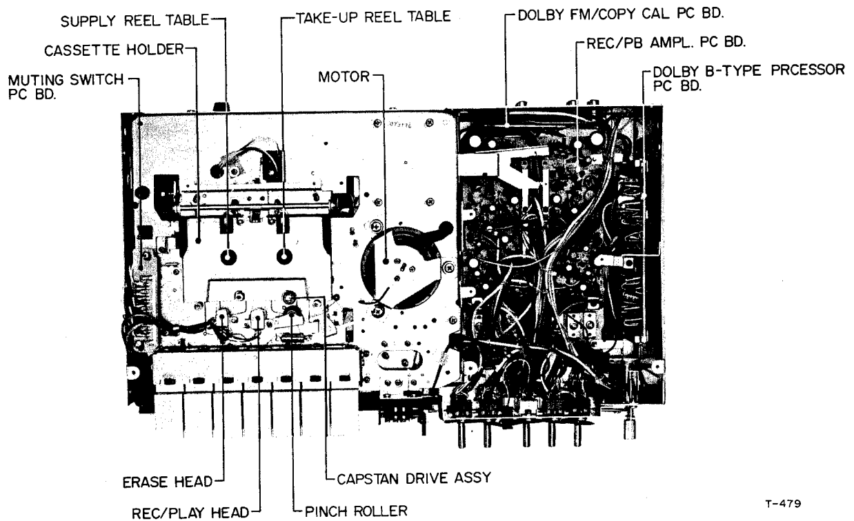
Fig. 5-2 Top View
