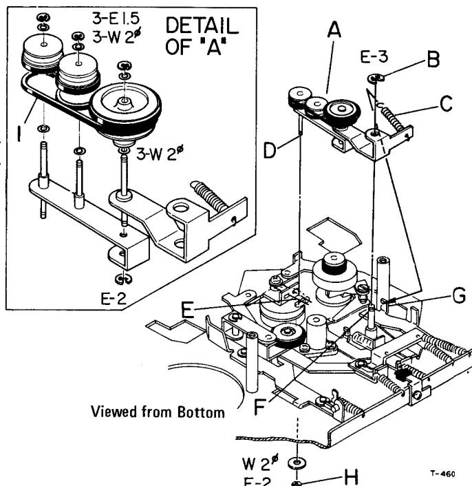
Fig. 3-10 Fast Wind Roller Ass'y Replacement
