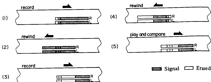
Fig. 7-19 Erase Efficiency Check Procedure
