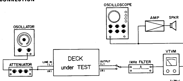
Fig. 7-18 Connection
