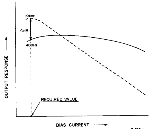
Fig. 7-13 Bias Adjustments (Hi-Fi tape)
