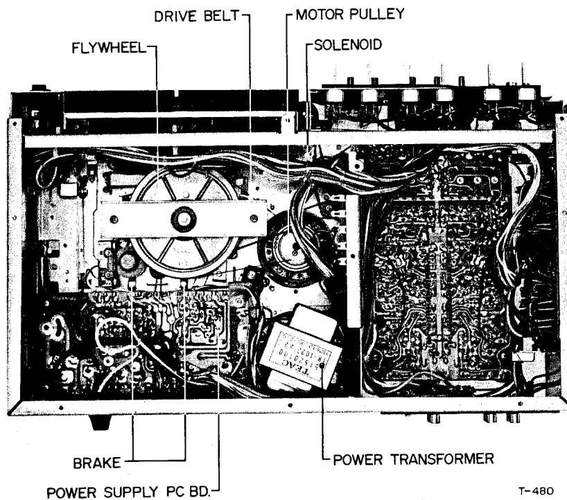
Fig. 5-3 Bottom View
