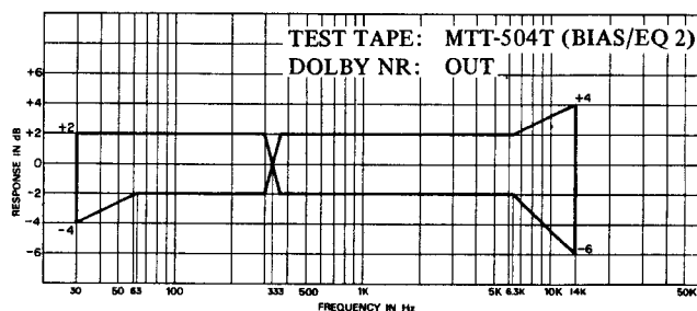
Fig. 7-16 Overall Frequency Response Limits (for BIAS/EQ 2)
