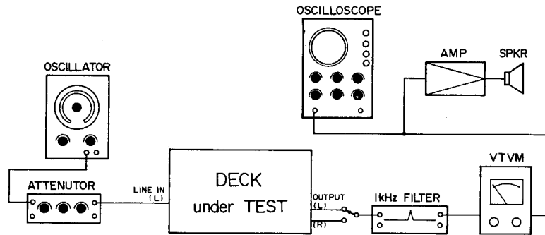
Fig. 7-20 Connection
