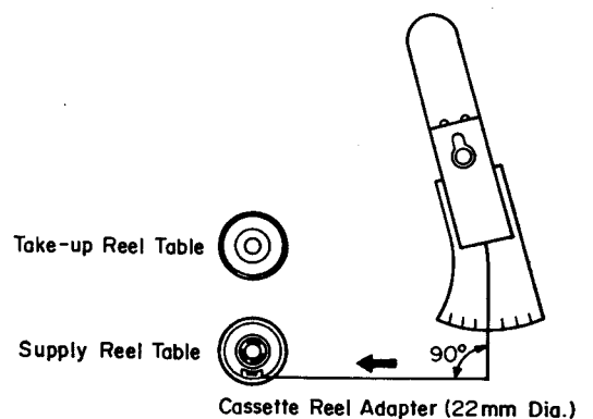
Fig. 4-4 Rewind Torque Measurement
