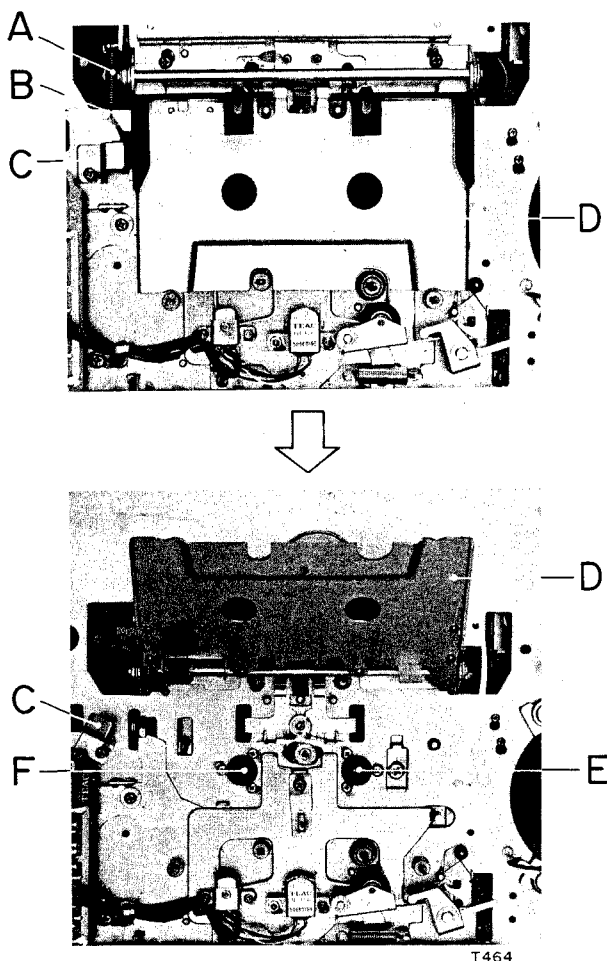
Fig. 3-8 Rotation of Cassette Holder
