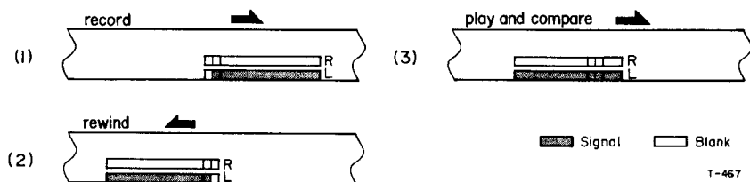
Fig. 7-21 Channel Separation Check Procedure
