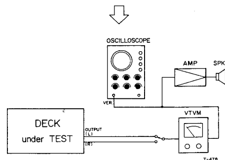
Fig. 7-4 Connections
