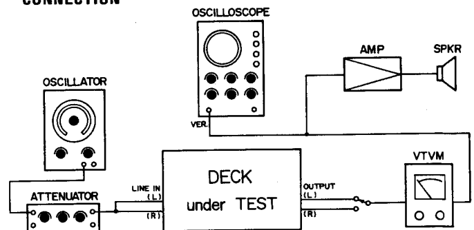
Fig. 7-10 Connection
