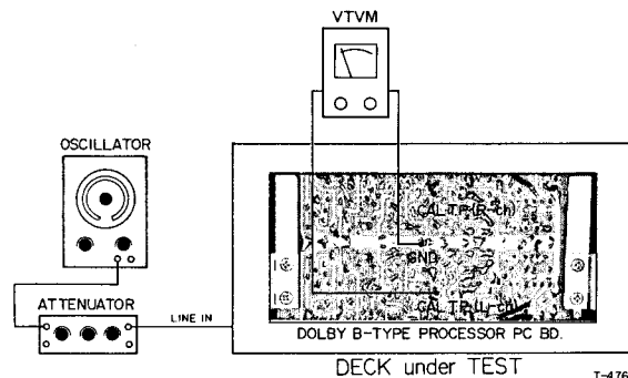
Fig. 7-8 Connection
