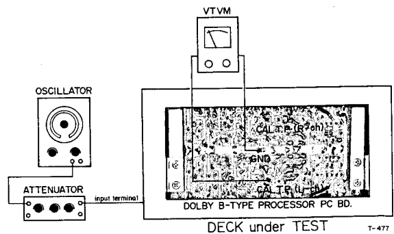
Fig. 7-7 Connection
