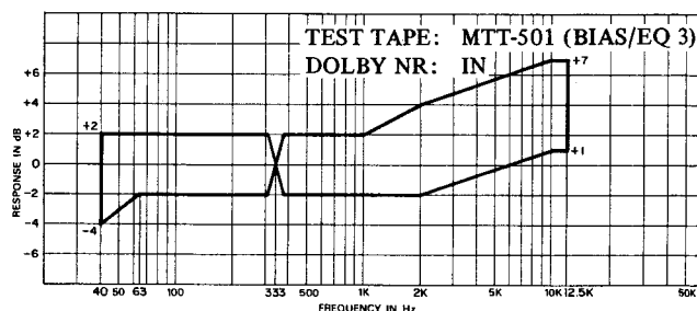
Fig. 7-17 Overall Frequency Response Limits (for BIAS/EQ 3)
