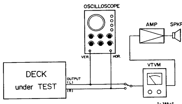
Fig. 7-3 Connection
