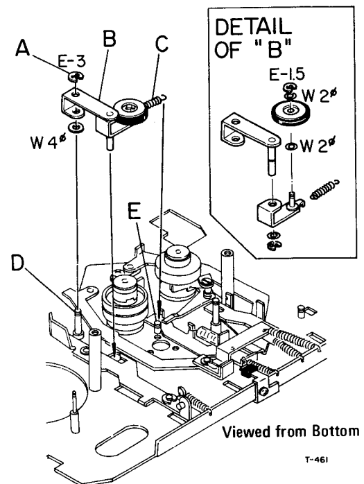
Fig. 3-12 Play Idler Ass'y Replacement
