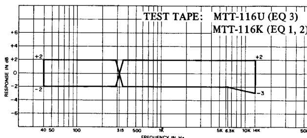
Fig. 7-5 Playback Frequency Response Limits
