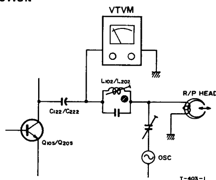
Fig. 7-11 Connection
