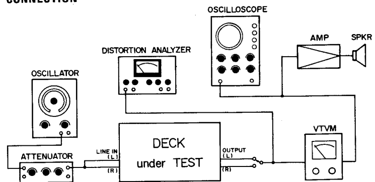
Fig. 7-14 Connection
